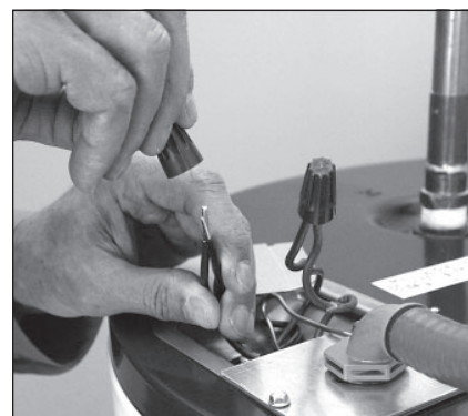
Figure 19 - Connecting the electrical wires.
